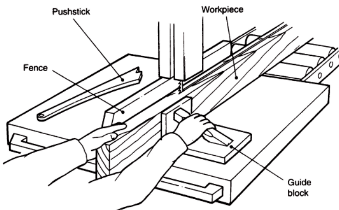
Figure 2 Straight cutting
