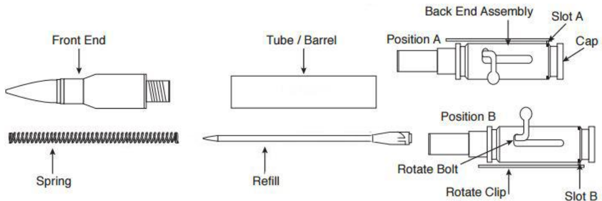
Diagram 1 – The Parts of the Pen included in the Kit
