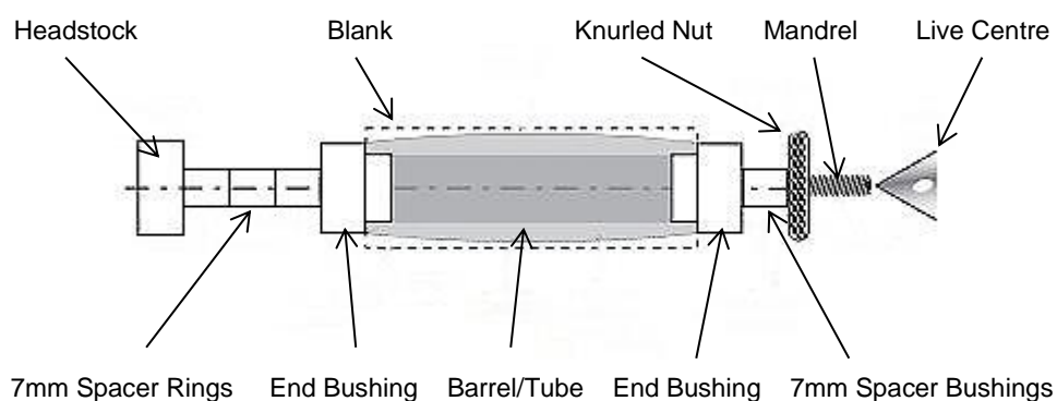
Diagram 2 – Mandrel Assembly
